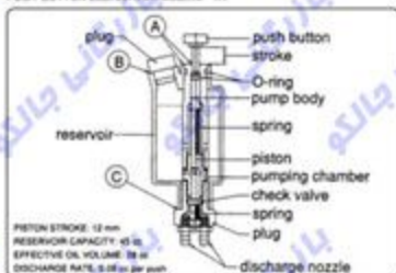
PUSH-BUTTON LUBRICATOR Model NP-7A
